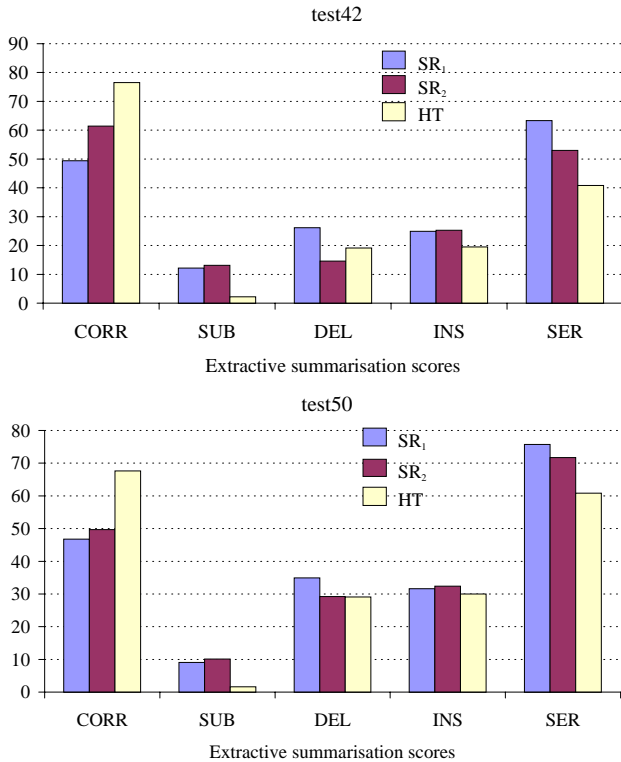
Figure 2: Extractive summarization scores on test42 and test50 for SR 1 , SR 2 and human transcription (HT) input, respectively.
