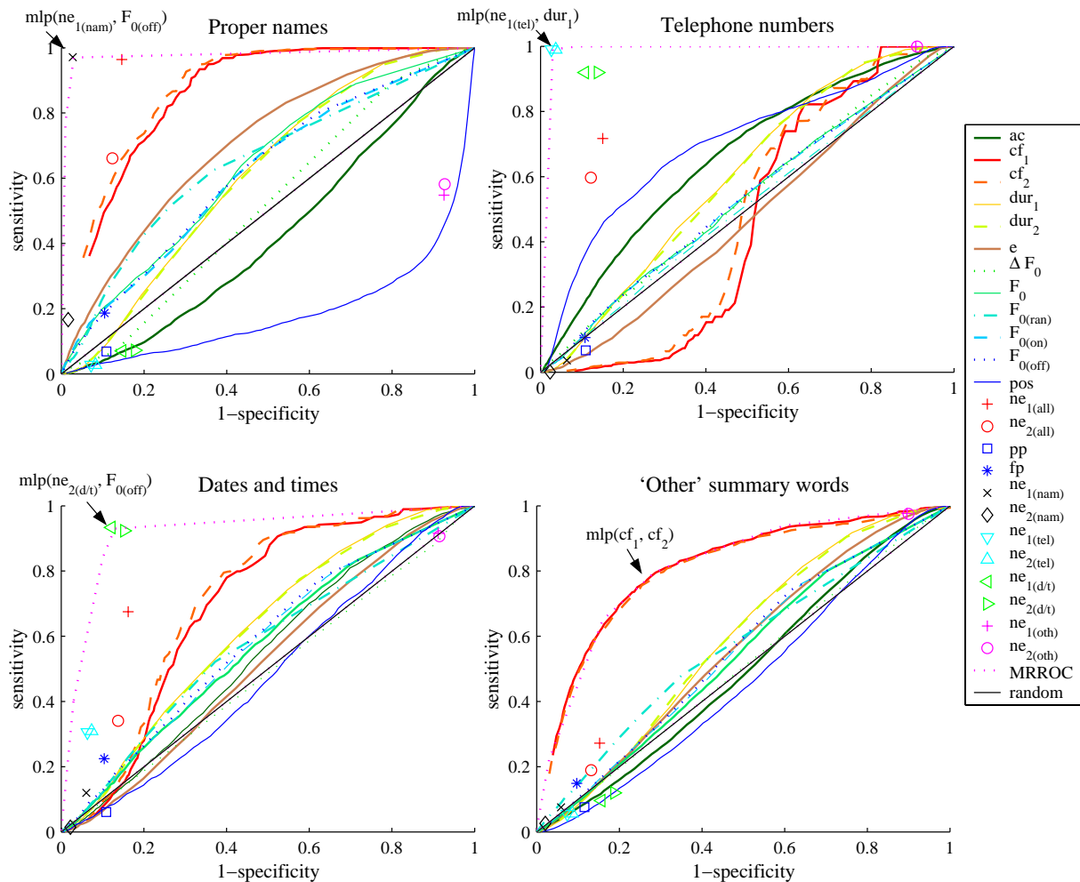
Figure 1: The ROC curves produced for the multi-class summarisation task using the individual features listed in Table 2 as inputs to a linear classifier with respect to the validation set. The MRROC curves produced by Parcel are also shown, along with the input features to MLPs at the MRROC vertex closer to the optimal classifier.
